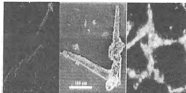
Figure Precambrian sponge spicules preserved in Late Proterozoic dolomites of the Yangtze Gorges area, South China.
