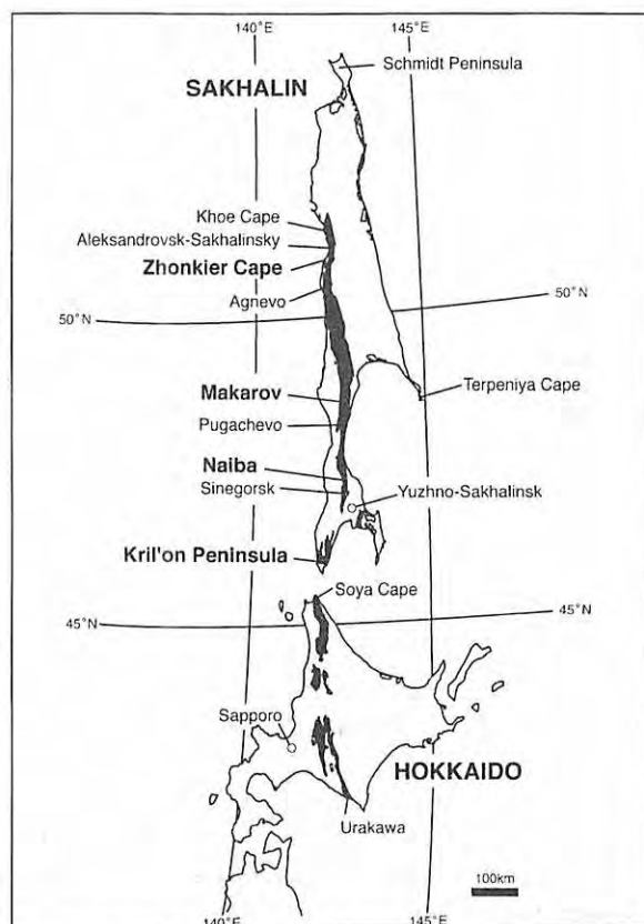
図1. 蝦夷層群分布図 [Shigeta and Maeda, 2005]
