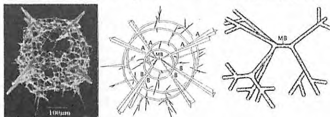
Fig.1 SEM photo of a species of family Polyentactiniidae from lateral view (left) and drawing of its initial spicule system (middle); the initial spicules of a species of family Entactiniidae (right). -Abbreviations: MB- median bar, A- apical spine, B- basal spine.
